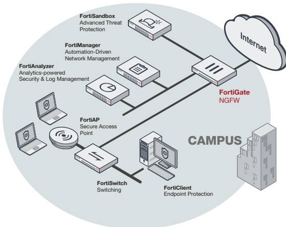
FortiGate 200F deployment in Campus (NGFW)
